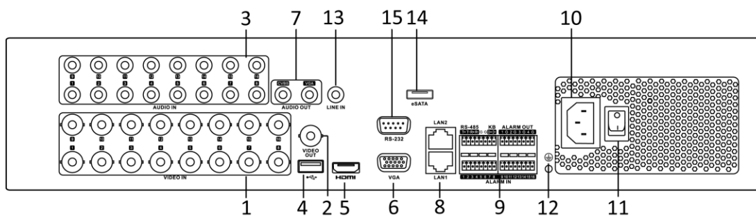
Figure 1. 16 DS-8100HQHI-SH
