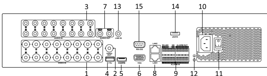
Figure 1. 14 DS-8116HGHI-SH
