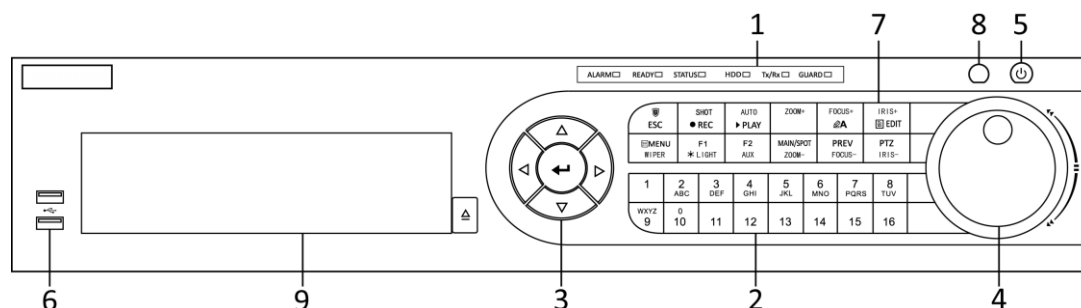
Figure 1. 6 Front Panel of DS-8100HGHI-SH and DS-8100HQHI-SH
