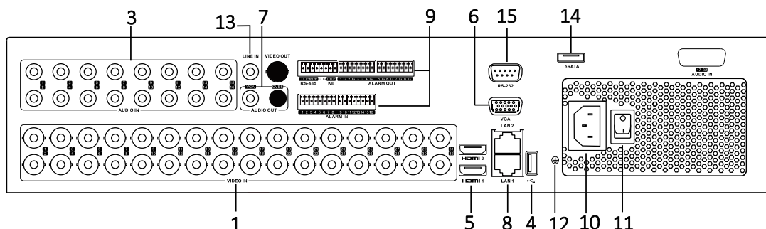
Figure 1. 15 DS-8132HGHI-SH
